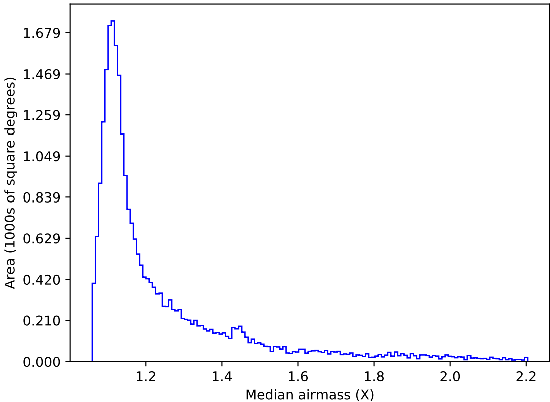
too_elab_r64_d2_gz_v3.4_10yrs Yr 1 i band: Median airmass
