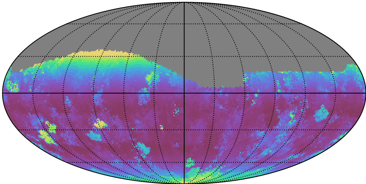
too_elab_r64_d2_gz_v3.4_10yrs Yr 1 g band: Median airmass
