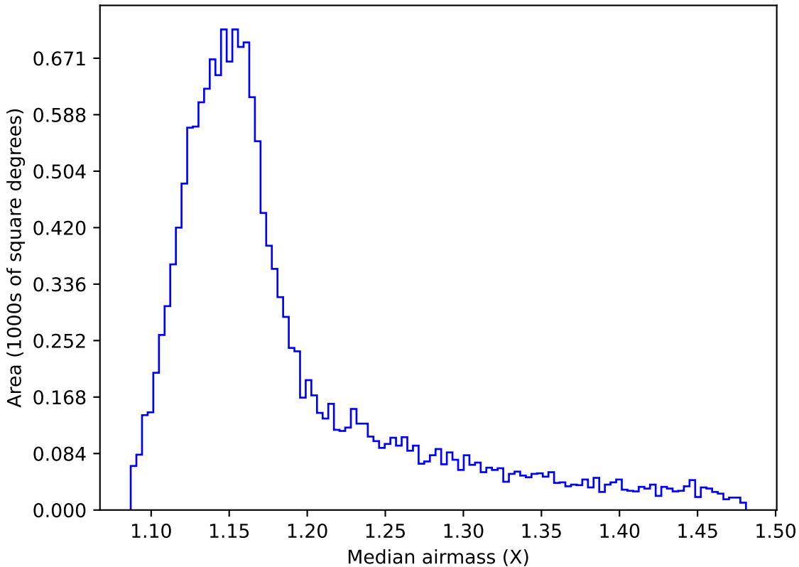
too_elab_r64_d2_gz_v3.4_10yrs WFD z band: Median airmass
