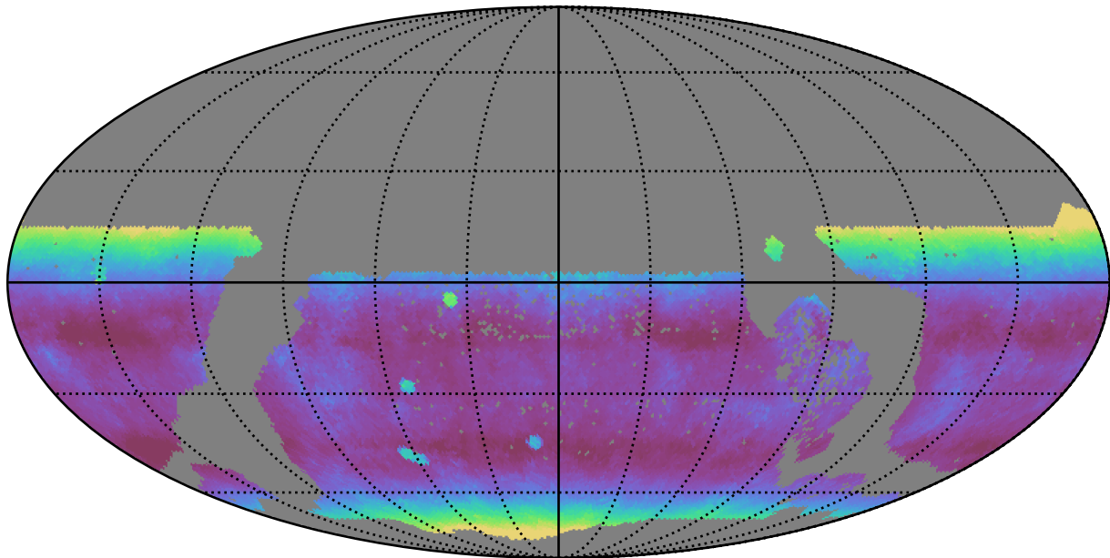
too_elab_r64_d2_gz_v3.4_10yrs WFD y band: Median airmass
