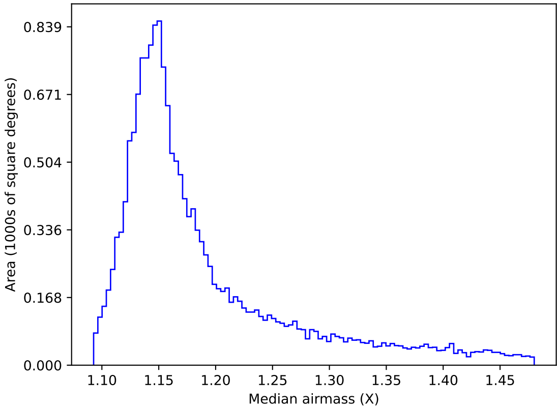
too_elab_r64_d2_gz_v3.4_10yrs WFD y band: Median airmass
