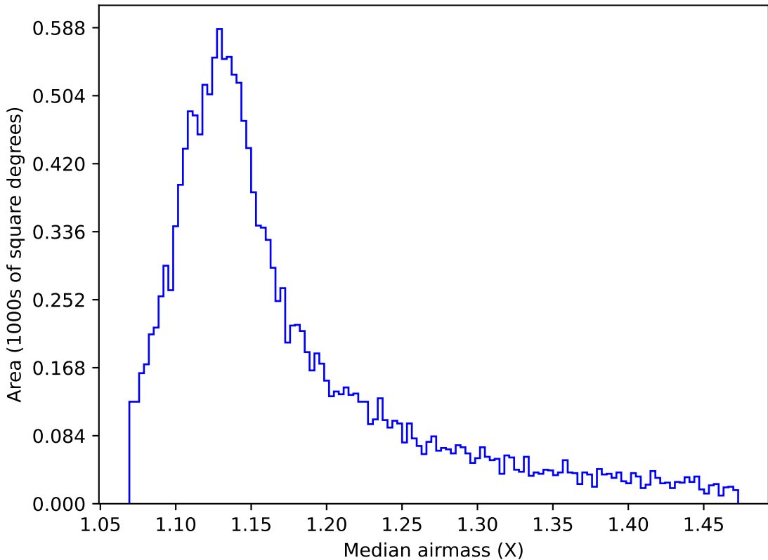
too_elab_r64_d2_gz_v3.4_10yrs WFD u band: Median airmass
