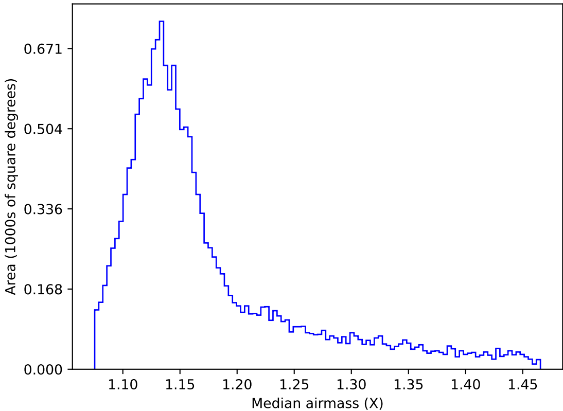
too_elab_r64_d2_gz_v3.4_10yrs WFD r band: Median airmass
