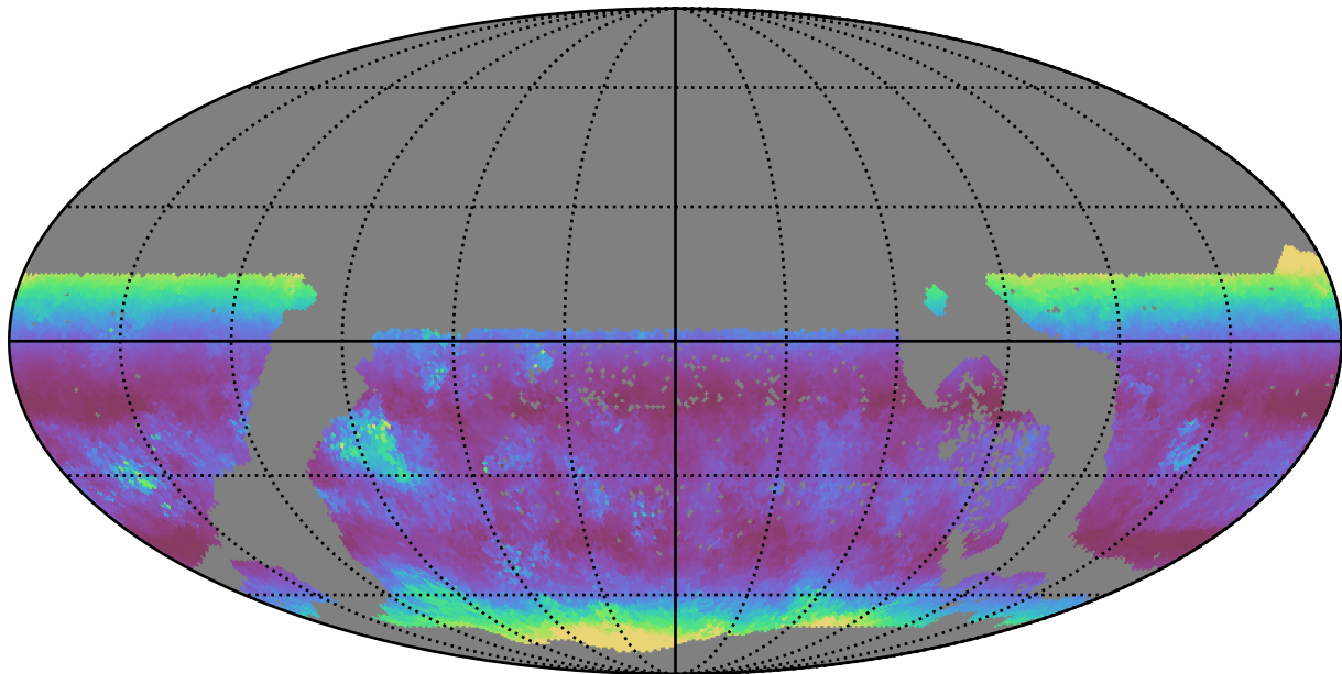
too_elab_r64_d2_gz_v3.4_10yrs WFD g band: Median airmass
