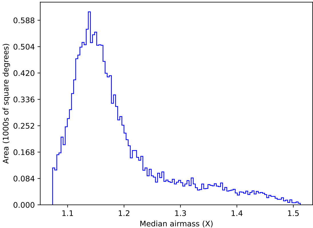
too_elab_r64_d2_gz_v3.4_10yrs WFD g band: Median airmass
