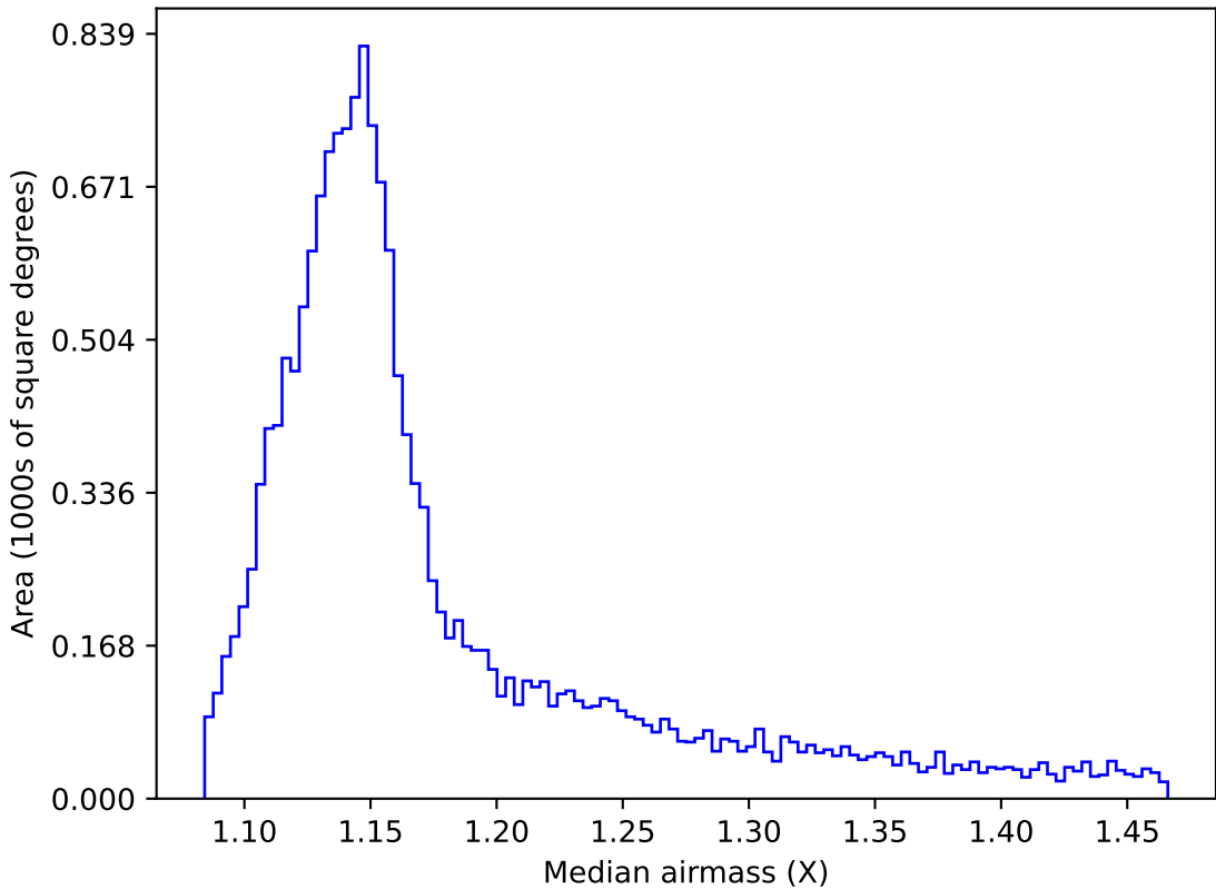
too_elab_r64_d2_gz_v3.4_10yrs WFD all bands: Median airmass
