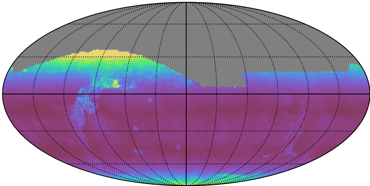
too_elab_r64_d2_gz_v3.4_10yrs All sky z band: Median airmass
