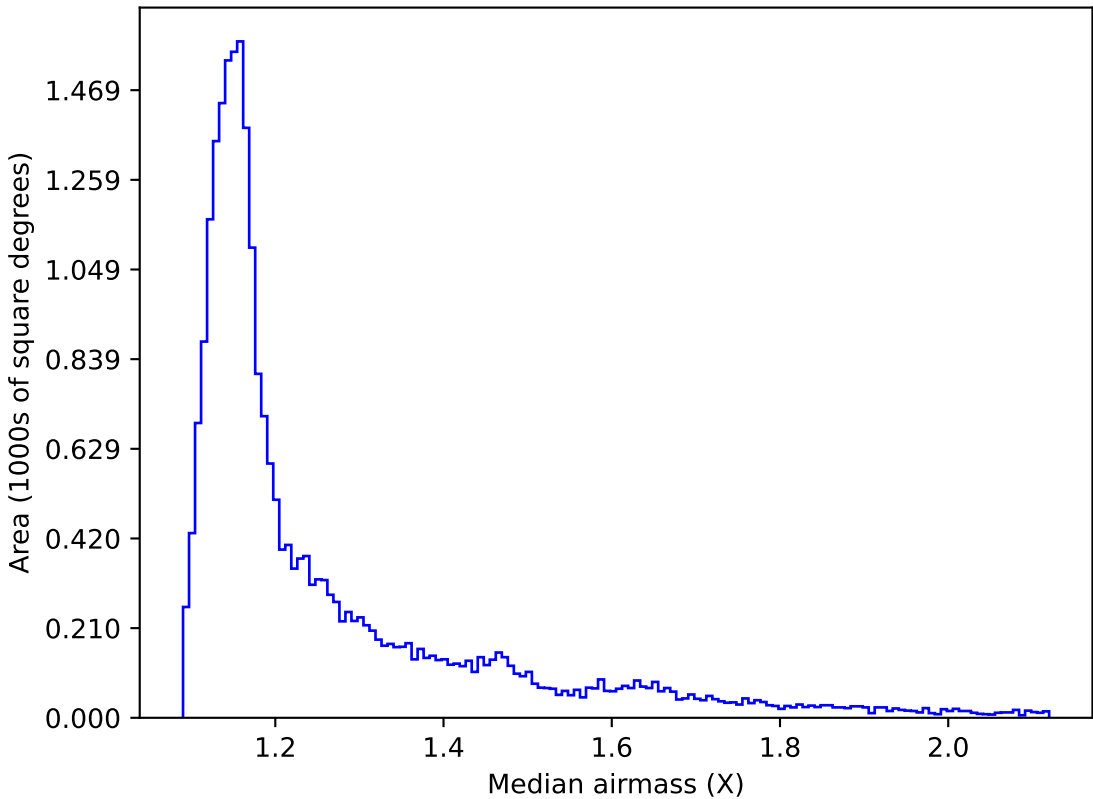
too_elab_r64_d2_gz_v3.4_10yrs All sky z band: Median airmass
