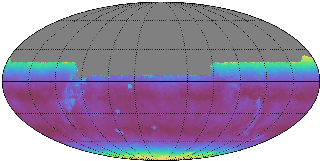
too_elab_r64_d2_gz_v3.4_10yrs All sky y band: Median airmass
