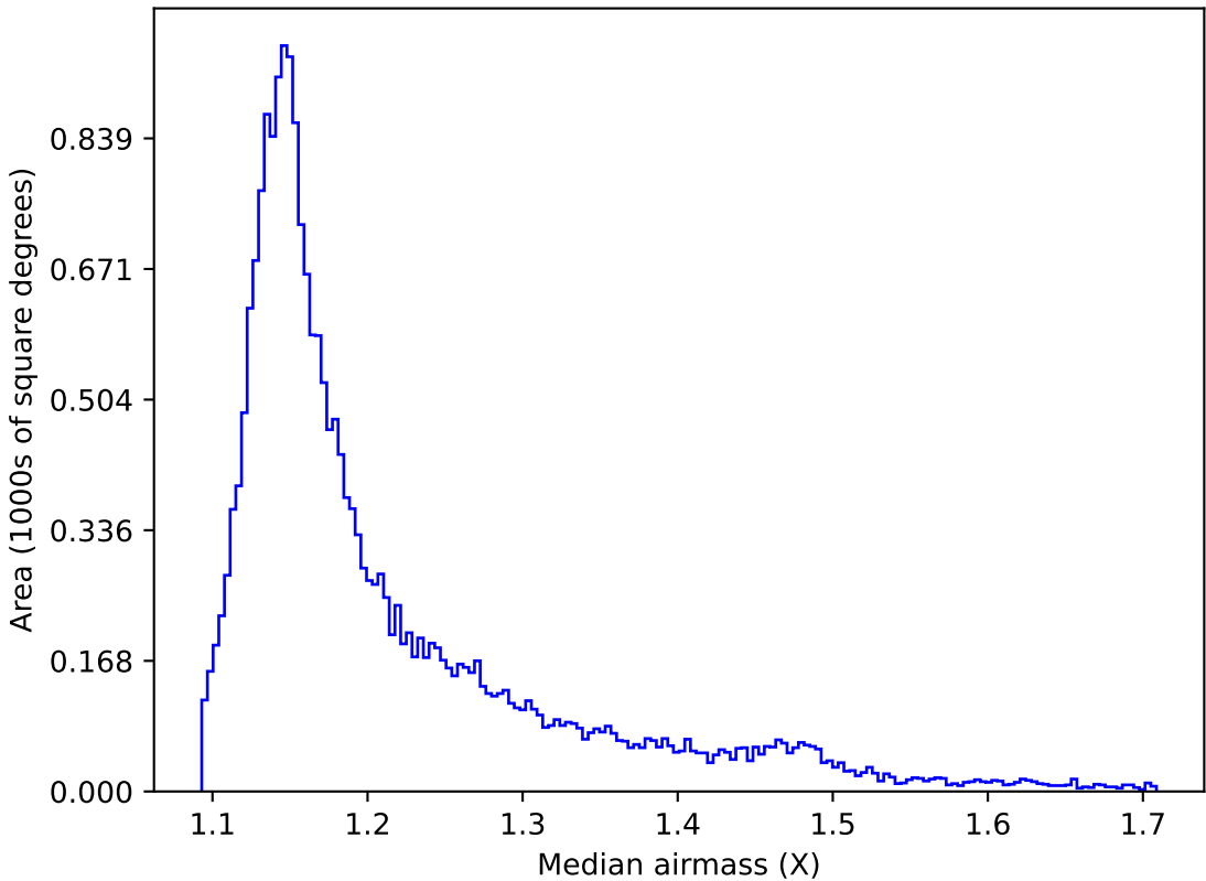
too_elab_r64_d2_gz_v3.4_10yrs All sky y band: Median airmass
