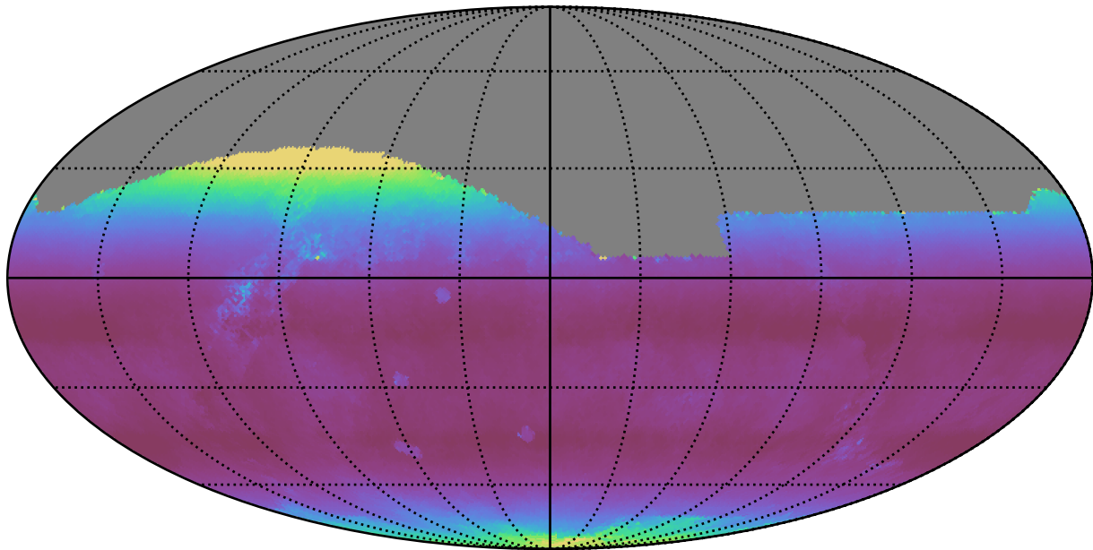
too_elab_r64_d2_gz_v3.4_10yrs All sky r band: Median airmass
