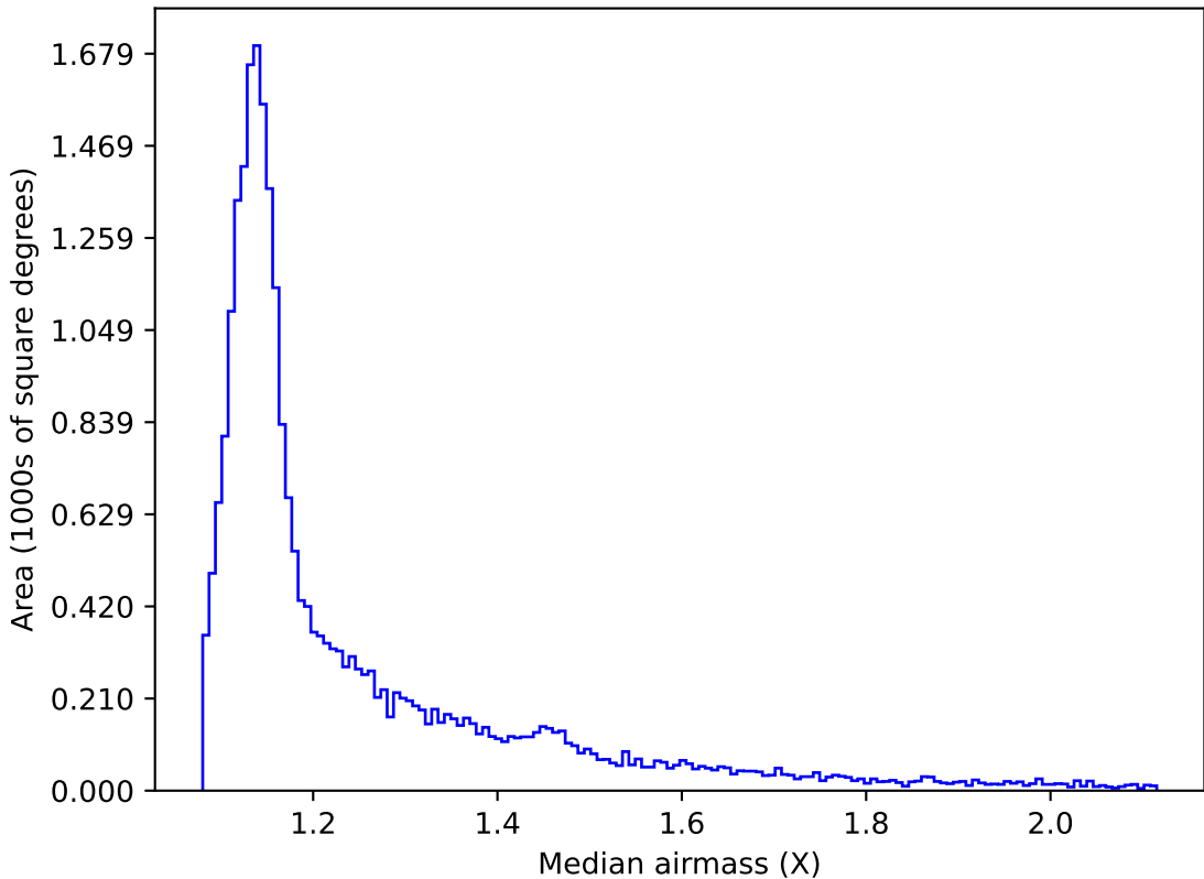
too_elab_r64_d2_gz_v3.4_10yrs All sky i band: Median airmass
