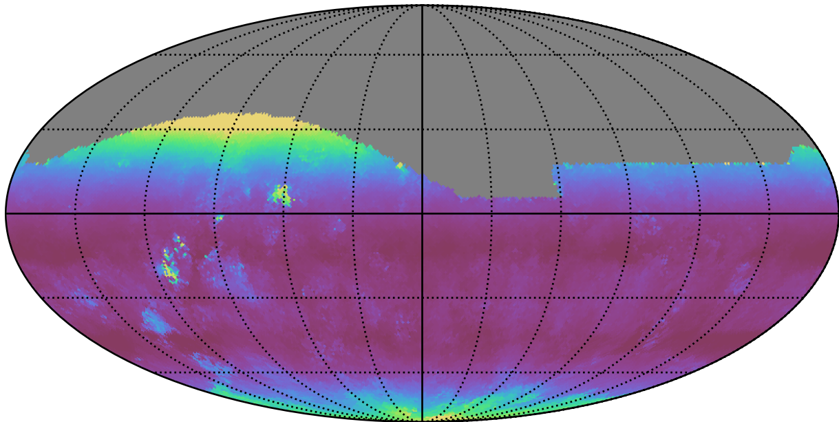
too_elab_r64_d2_gz_v3.4_10yrs All sky g band: Median airmass
