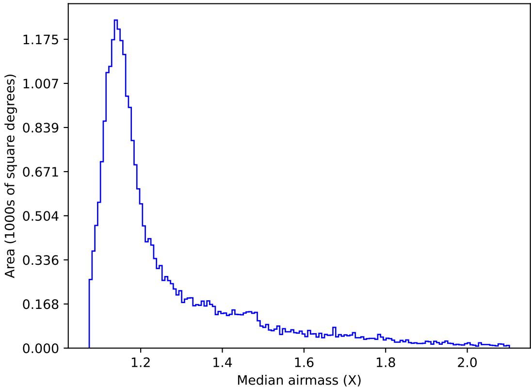
too_elab_r64_d2_gz_v3.4_10yrs All sky g band: Median airmass
