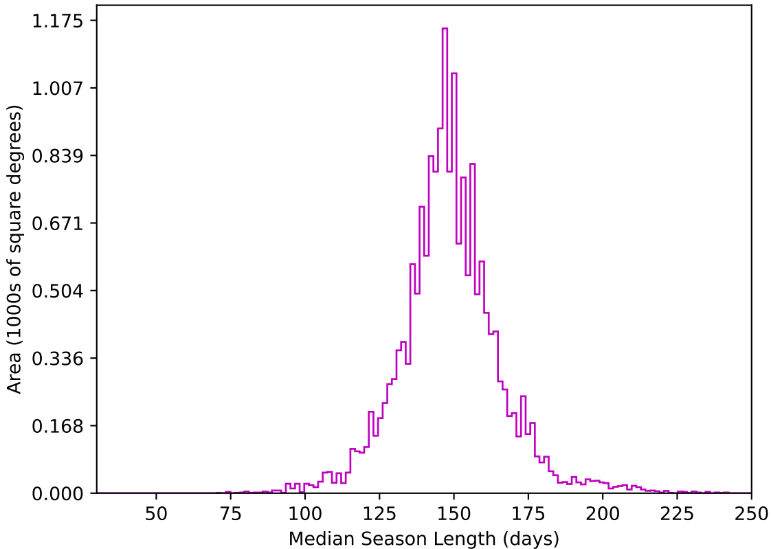
too_elab_r64_d2_gz_v3.4_10yrs WFD z band: Median Season Length
