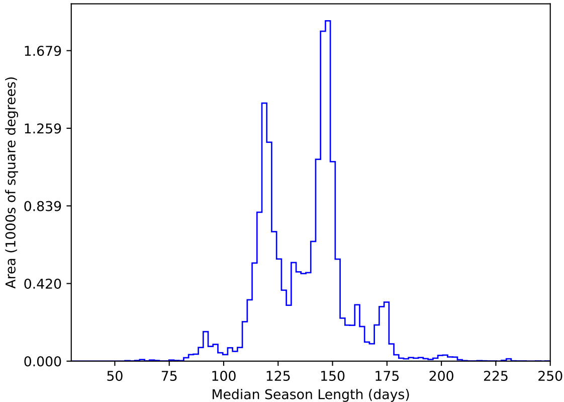
too_elab_r64_d2_gz_v3.4_10yrs WFD y band: Median Season Length
