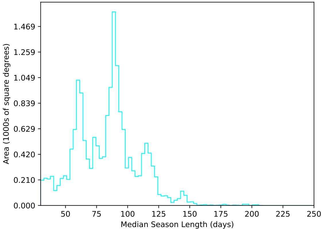
too_elab_r64_d2_gz_v3.4_10yrs WFD u band: Median Season Length
