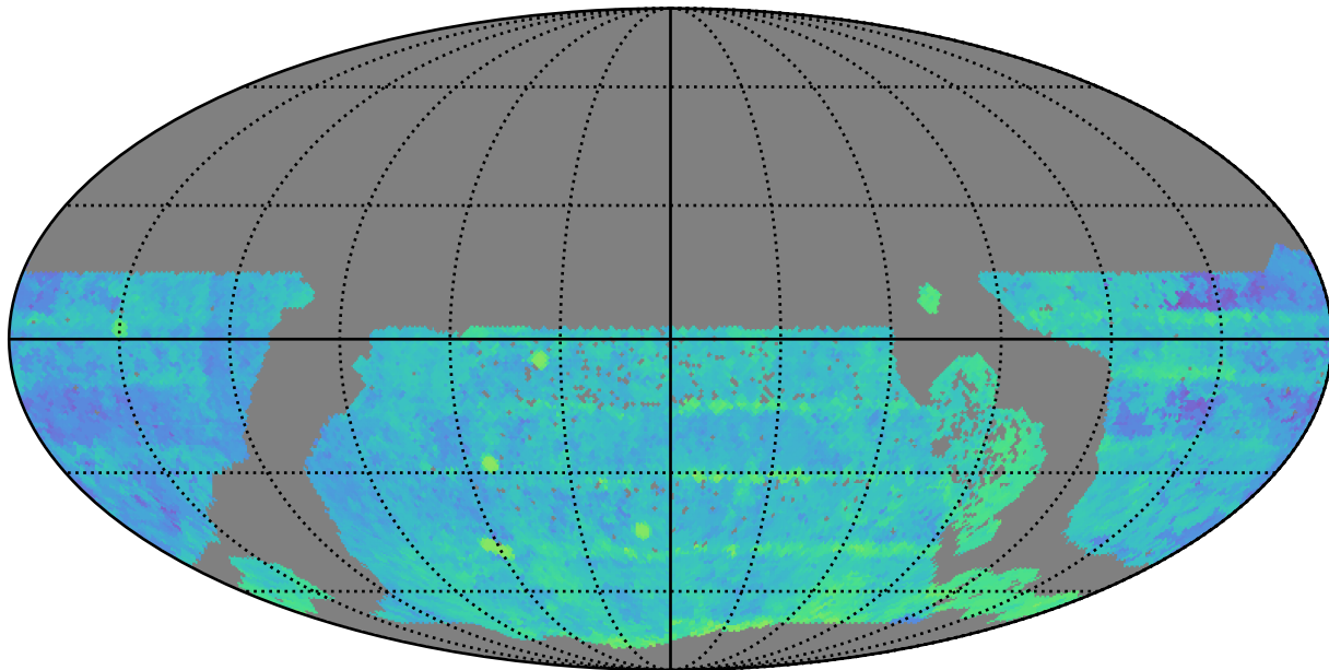
too_elab_r64_d2_gz_v3.4_10yrs WFD r band: Median Season Length
