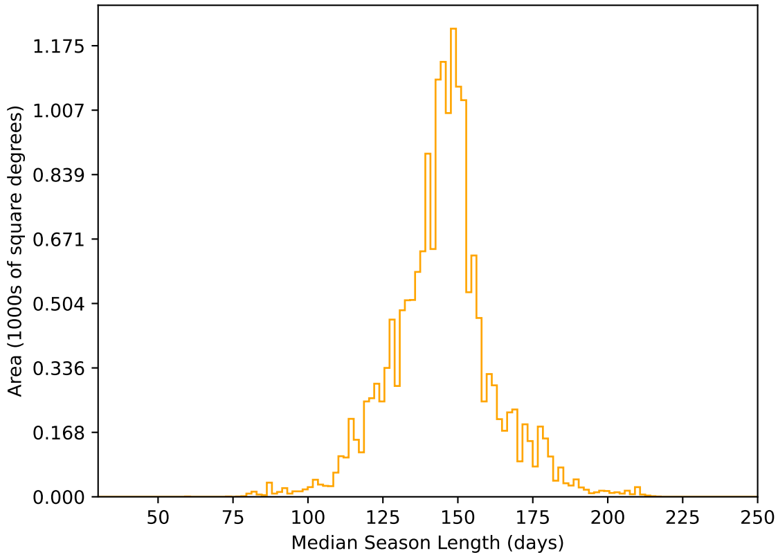
too_elab_r64_d2_gz_v3.4_10yrs WFD r band: Median Season Length
