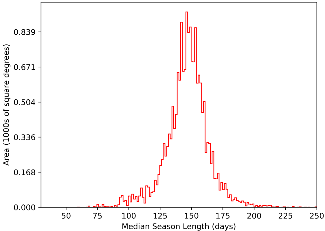
too_elab_r64_d2_gz_v3.4_10yrs WFD i band: Median Season Length
