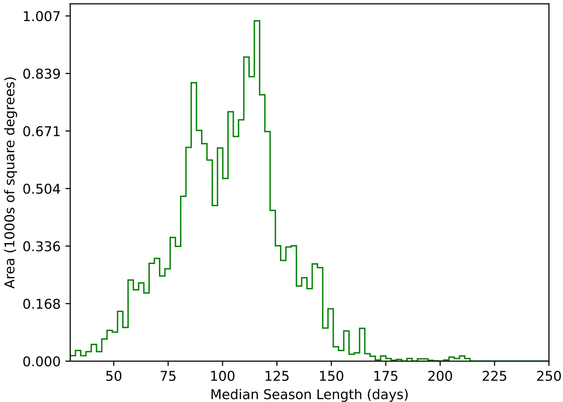
too_elab_r64_d2_gz_v3.4_10yrs WFD g band: Median Season Length
