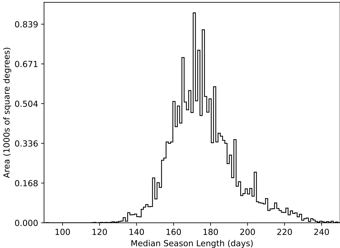
too_elab_r64_d2_gz_v3.4_10yrs WFD all bands: Median Season Length
