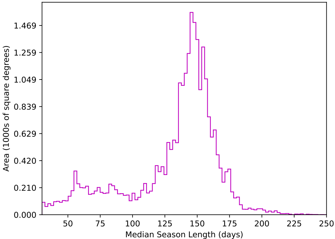
too_elab_r64_d2_gz_v3.4_10yrs All sky z band: Median Season Length
