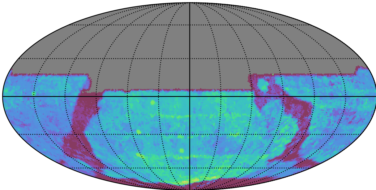
too_elab_r64_d2_gz_v3.4_10yrs All sky y band: Median Season Length
