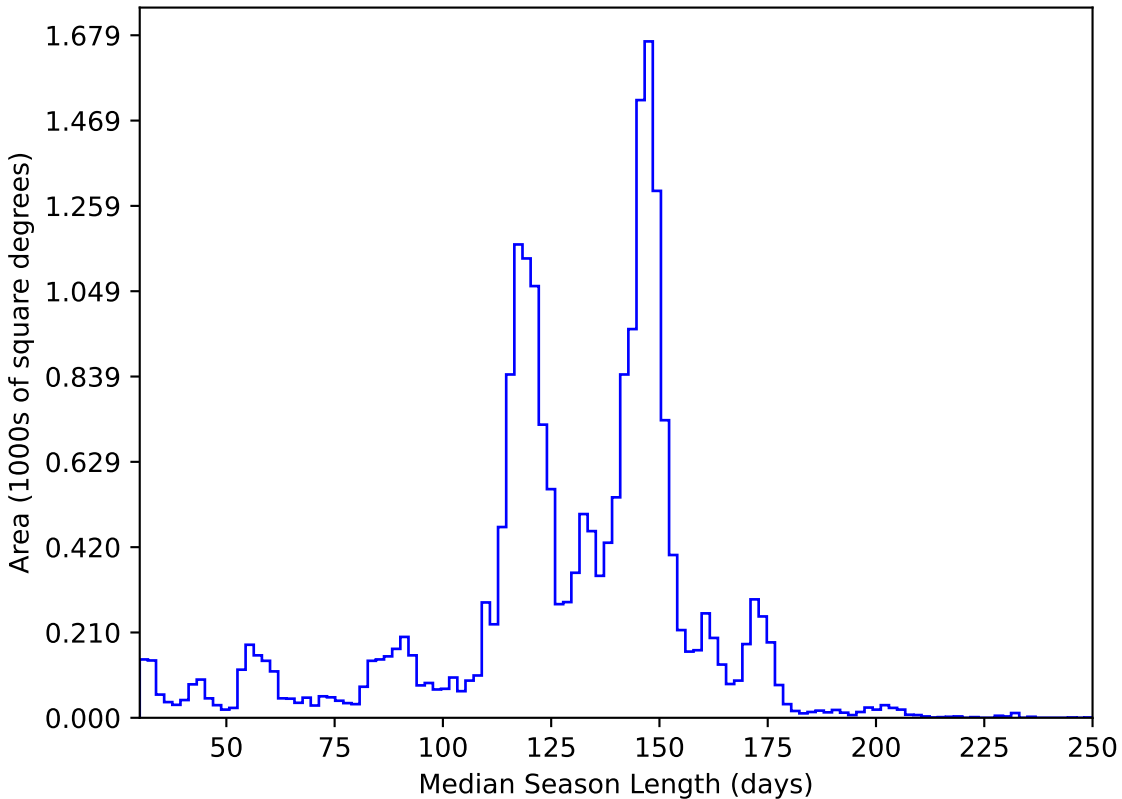
too_elab_r64_d2_gz_v3.4_10yrs All sky y band: Median Season Length
