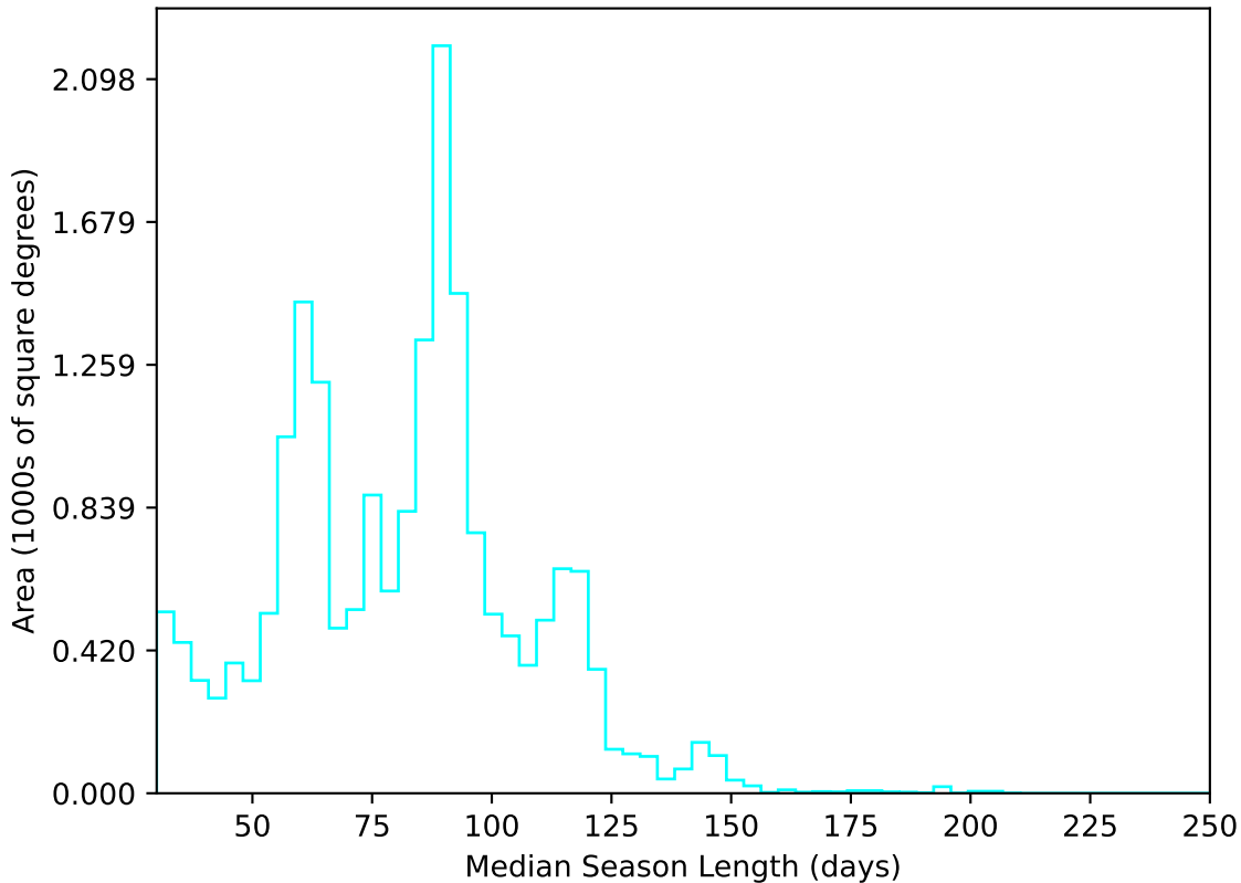
too_elab_r64_d2_gz_v3.4_10yrs All sky u band: Median Season Length
