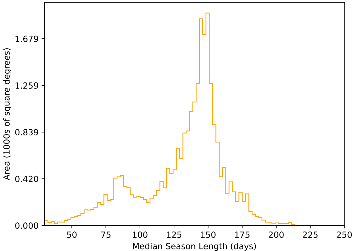
too_elab_r64_d2_gz_v3.4_10yrs All sky r band: Median Season Length
