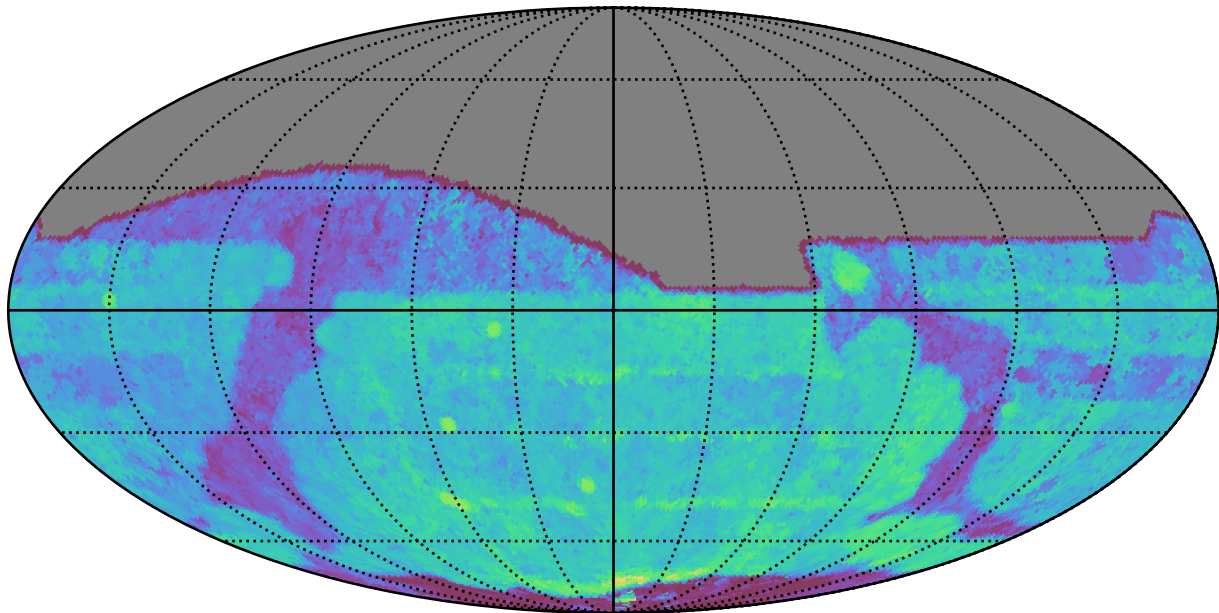
too_elab_r64_d2_gz_v3.4_10yrs All sky i band: Median Season Length
