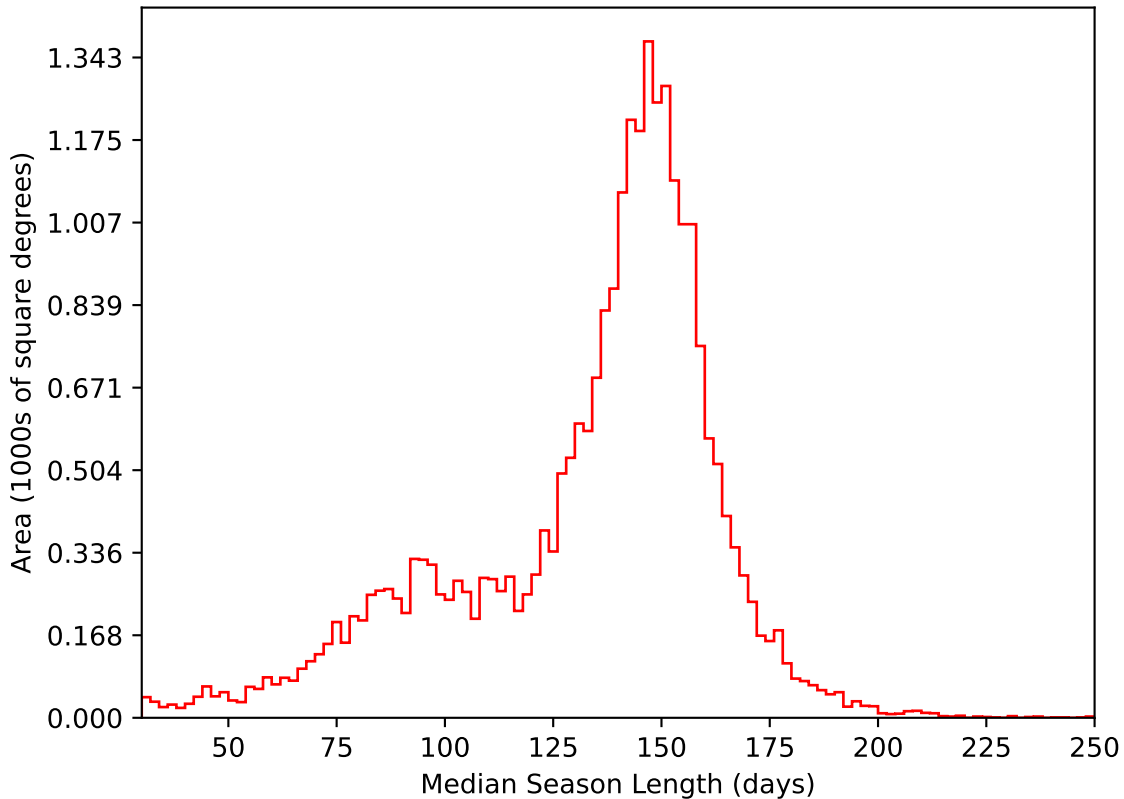
too_elab_r64_d2_gz_v3.4_10yrs All sky i band: Median Season Length
