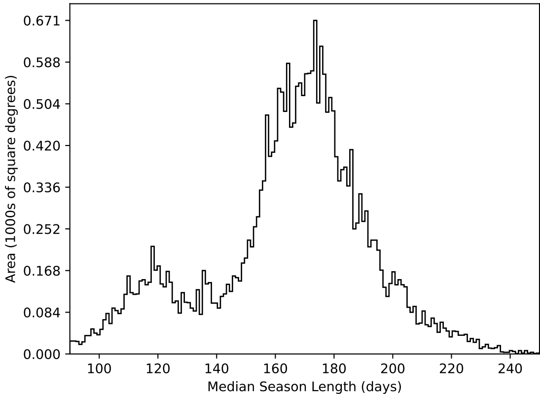
too_elab_r64_d2_gz_v3.4_10yrs All sky all bands: Median Season Length
