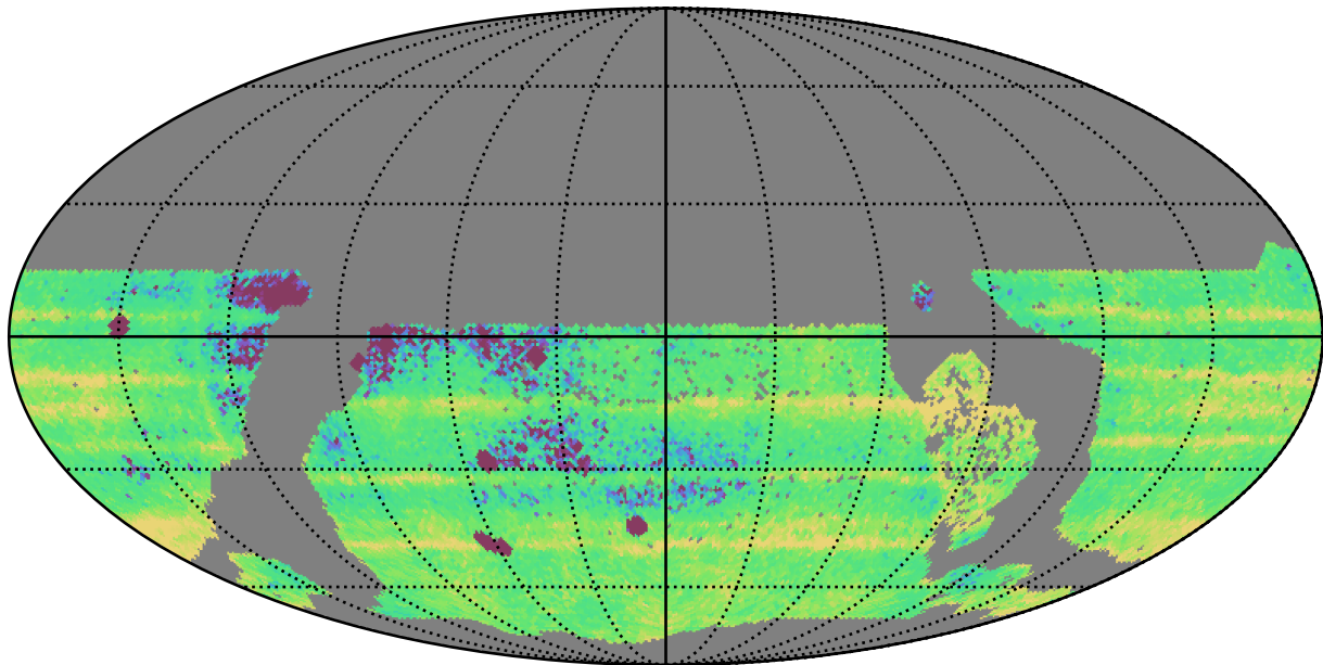
too_elab_r64_d2_gz_v3.4_10yrs WFD: Median Intra-Night Gap
