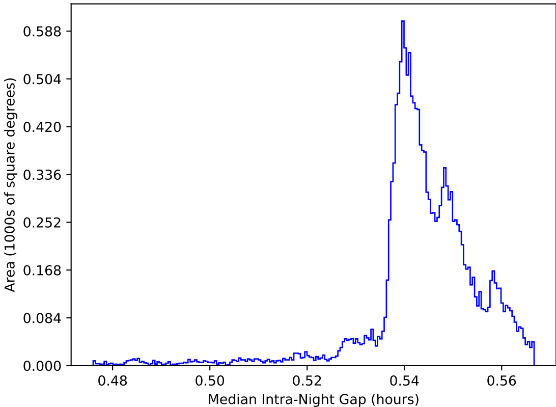
too_elab_r64_d2_gz_v3.4_10yrs WFD: Median Intra-Night Gap
