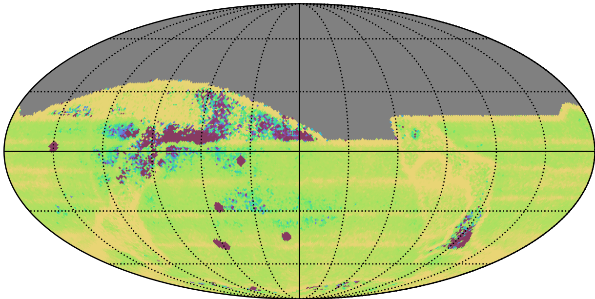
too_elab_r64_d2_gz_v3.4_10yrs All sky: Median Intra-Night Gap
