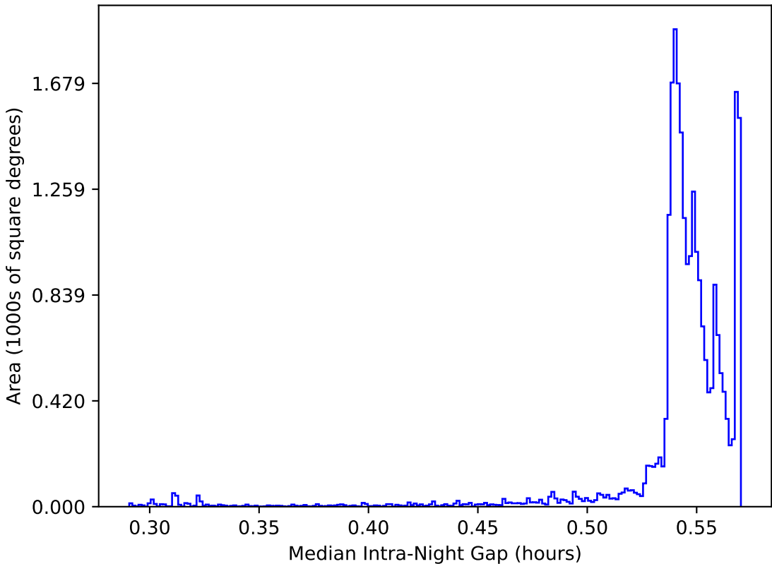
too_elab_r64_d2_gz_v3.4_10yrs All sky: Median Intra-Night Gap
