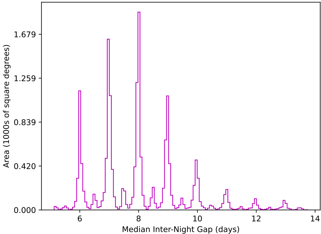
too_elab_r64_d2_gz_v3.4_10yrs WFD z band: Median Inter-Night Gap
