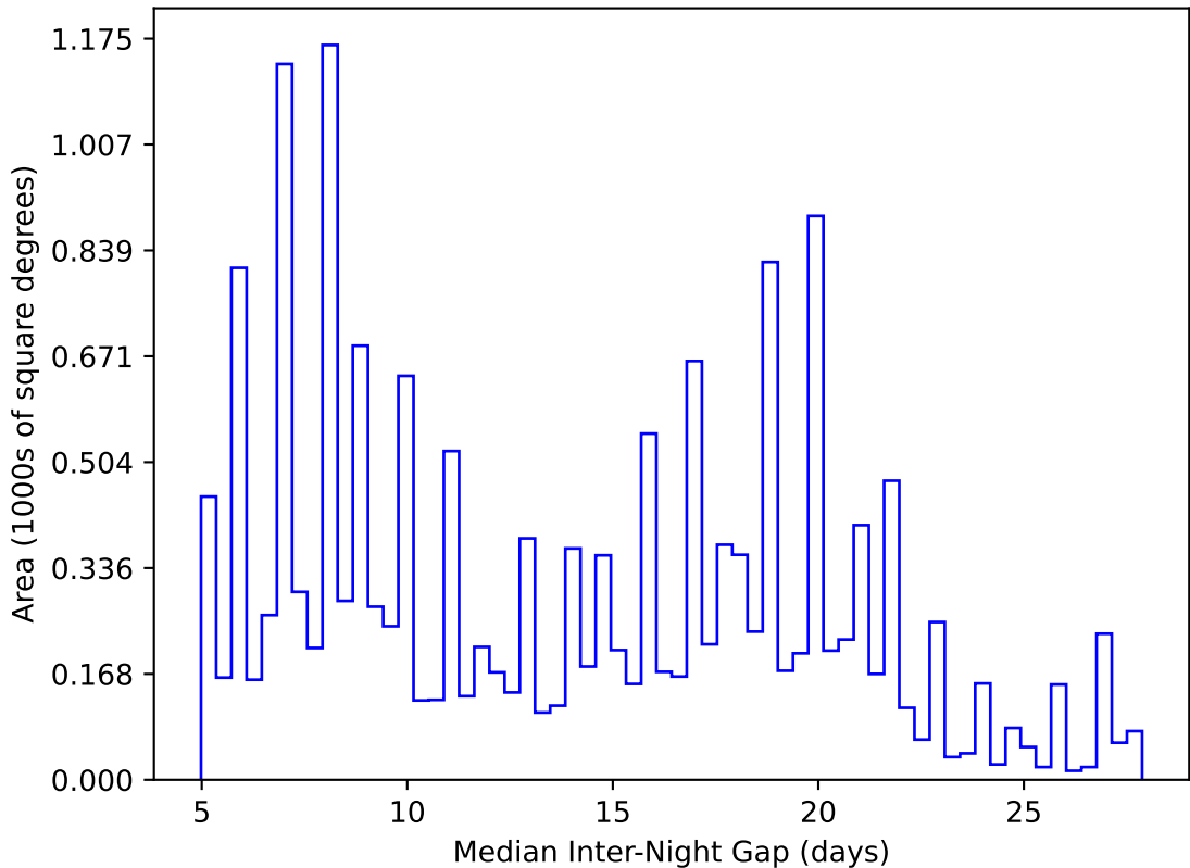
too_elab_r64_d2_gz_v3.4_10yrs WFD y band: Median Inter-Night Gap
