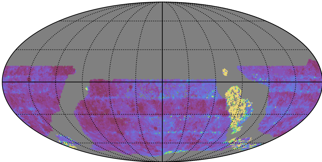
too_elab_r64_d2_gz_v3.4_10yrs WFD u band: Median Inter-Night Gap
