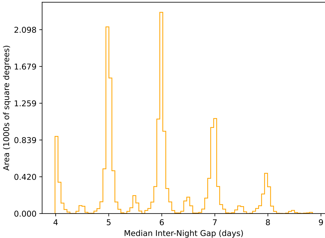
too_elab_r64_d2_gz_v3.4_10yrs WFD r band: Median Inter-Night Gap
