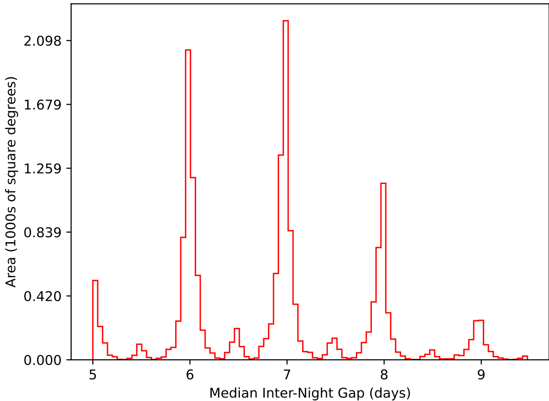
too_elab_r64_d2_gz_v3.4_10yrs WFD i band: Median Inter-Night Gap
