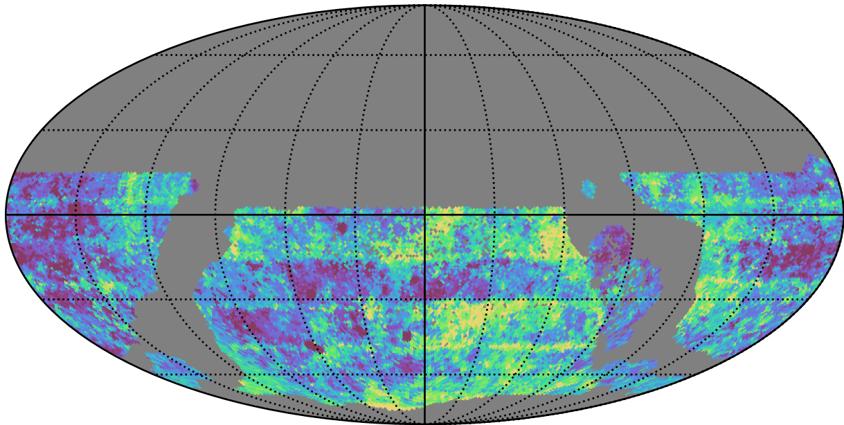
too_elab_r64_d2_gz_v3.4_10yrs WFD g band: Median Inter-Night Gap
