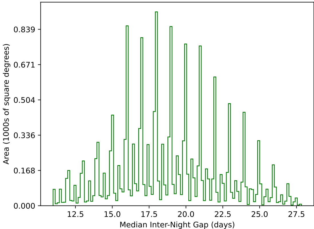
too_elab_r64_d2_gz_v3.4_10yrs WFD g band: Median Inter-Night Gap
