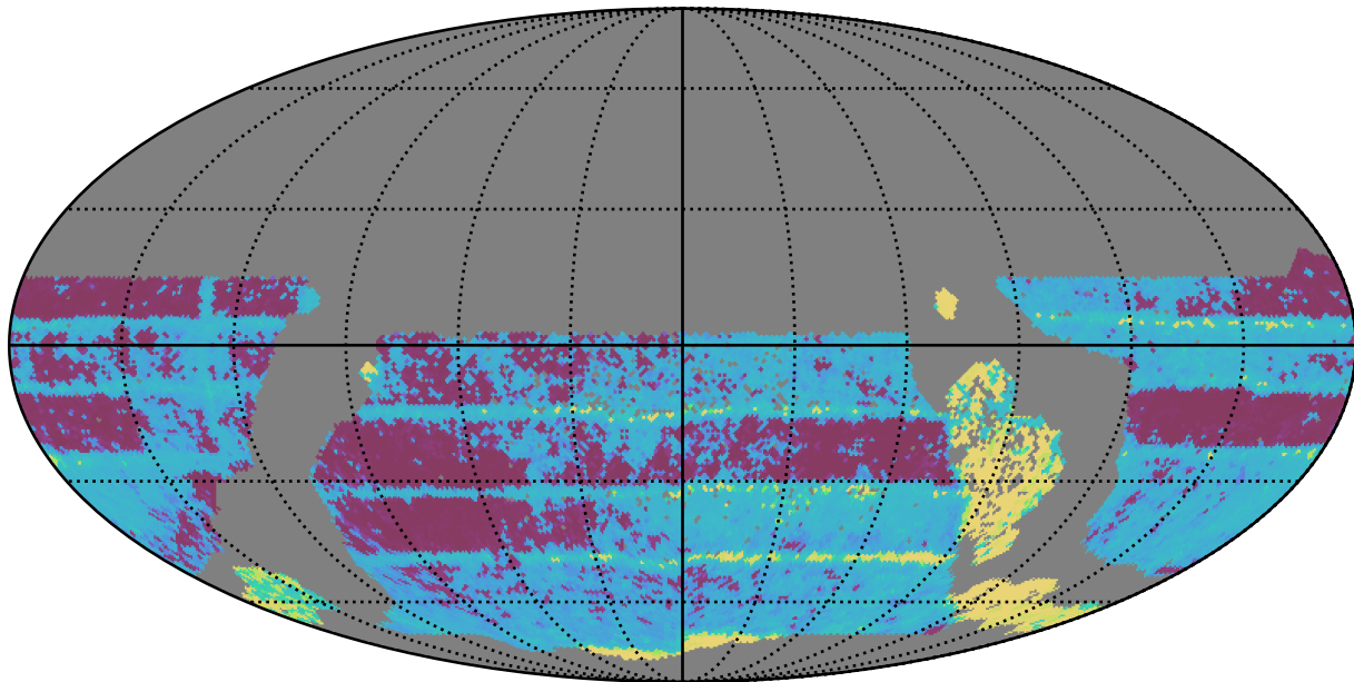
too_elab_r64_d2_gz_v3.4_10yrs WFD all bands: Median Inter-Night Gap
