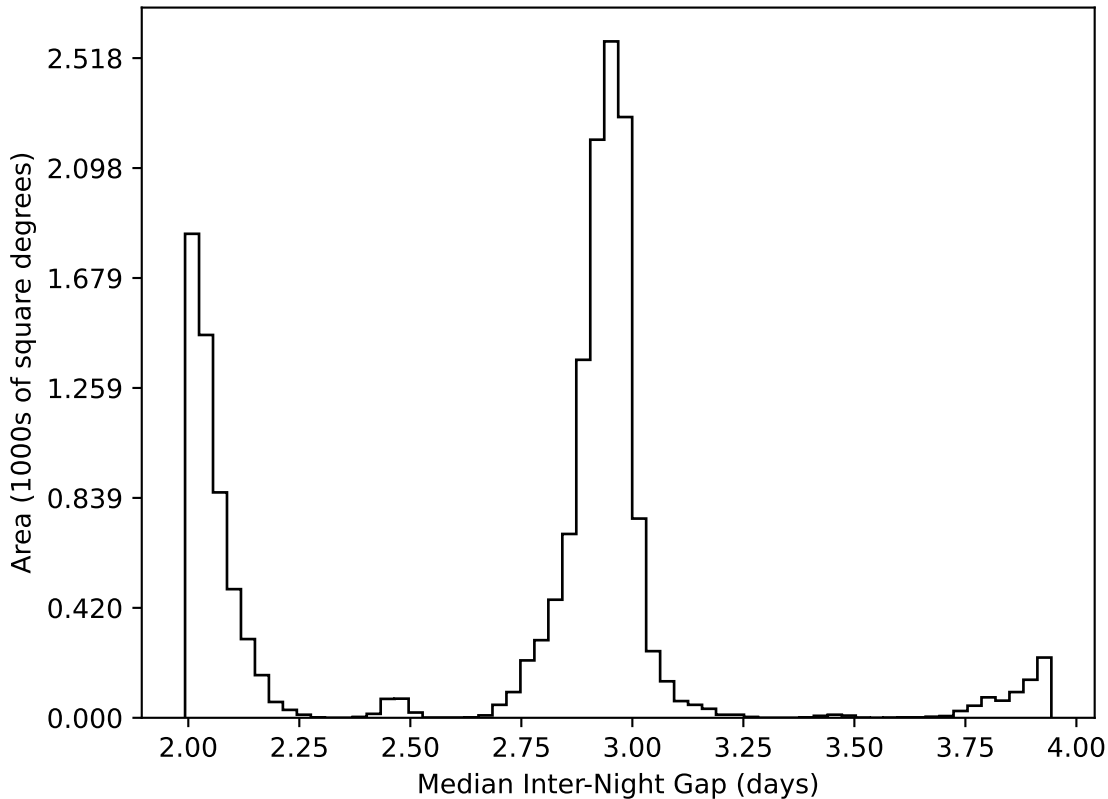
too_elab_r64_d2_gz_v3.4_10yrs WFD all bands: Median Inter-Night Gap
