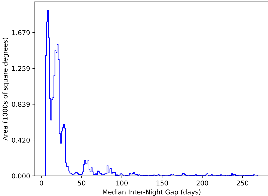
too_elab_r64_d2_gz_v3.4_10yrs All sky y band: Median Inter-Night Gap
