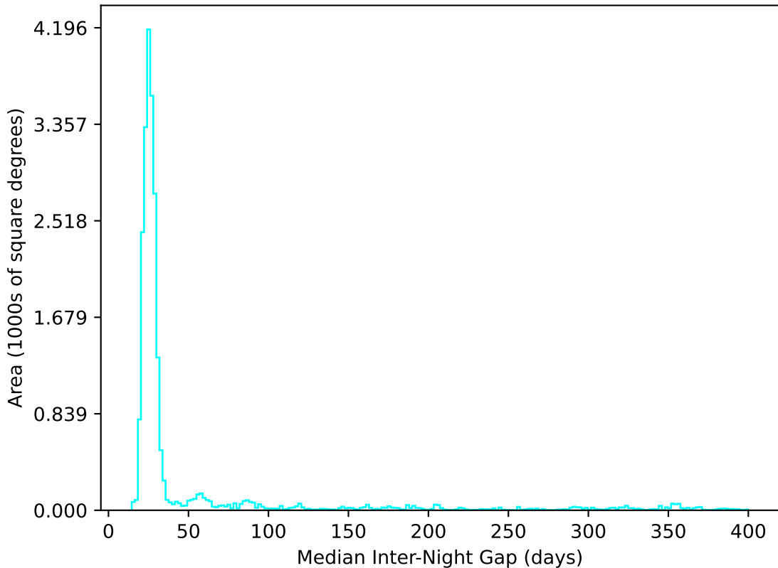
too_elab_r64_d2_gz_v3.4_10yrs All sky u band: Median Inter-Night Gap
