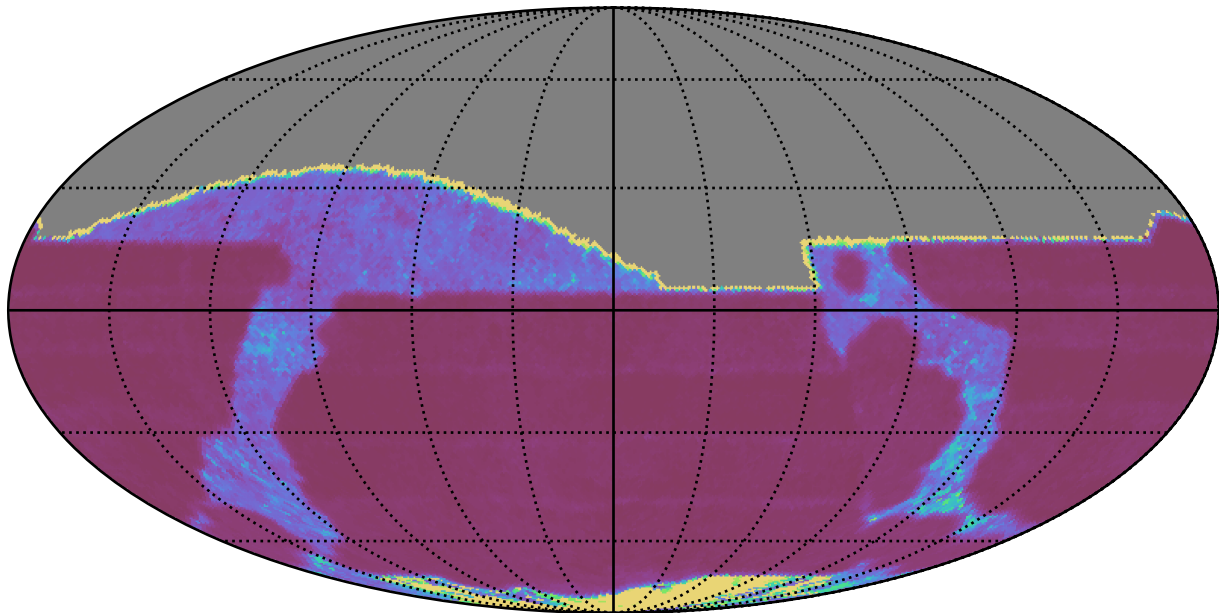
too_elab_r64_d2_gz_v3.4_10yrs All sky r band: Median Inter-Night Gap
